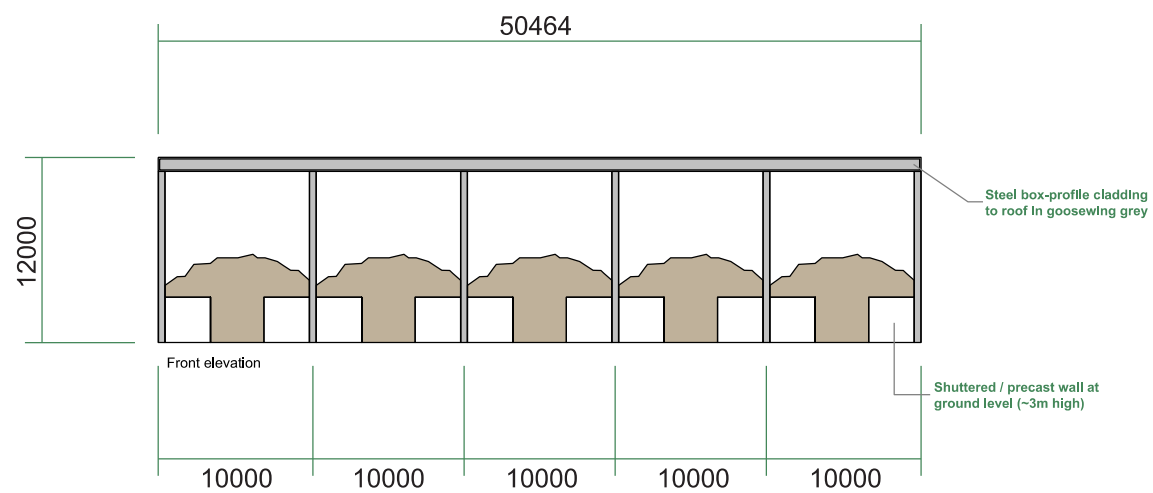
Front Elevation (Western)
