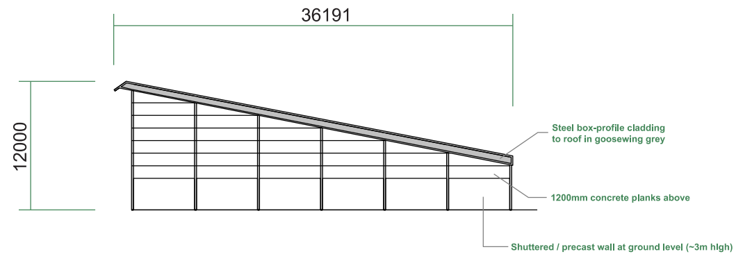
Side Elevation (North and South)
